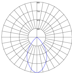
NOMINAL POLAR CURVE
